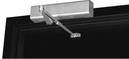
TPN arm shown (top jamb mounting)
