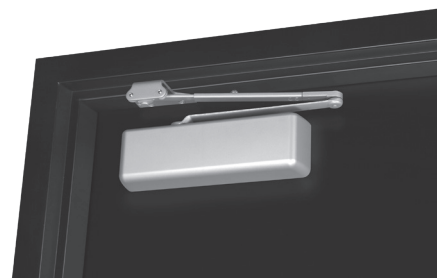
TPN arm shown (parallel mounting)
